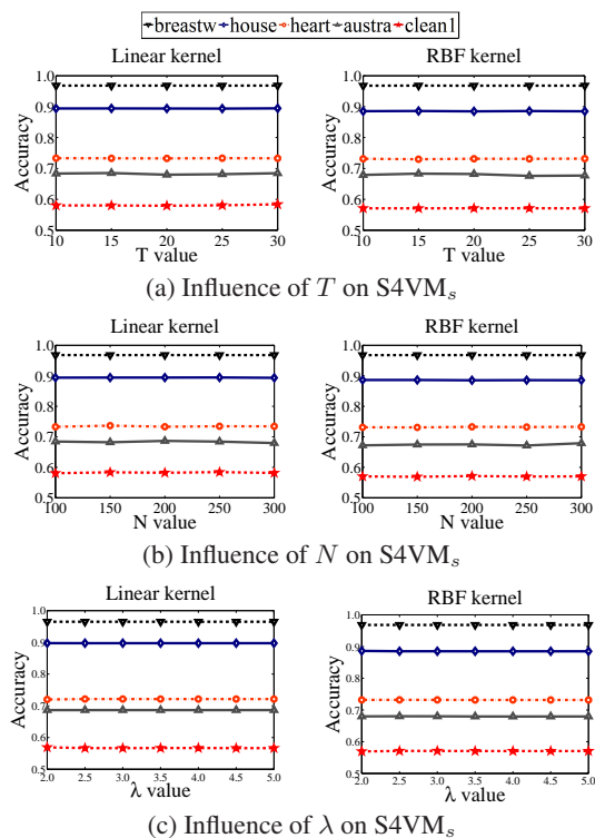
Figure 3. Parameter Influence with 10 labeled examples
