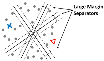
Figure 1. There are usually multiple large-margin low-density separators coincide well with labeled data (cross and triangle)
